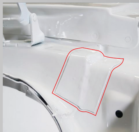
Paint Shop sealant tape on vehicle panel
