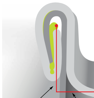
Schematic of Double Seaming
