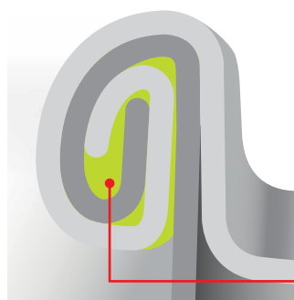
Schematic of Triple Seaming
